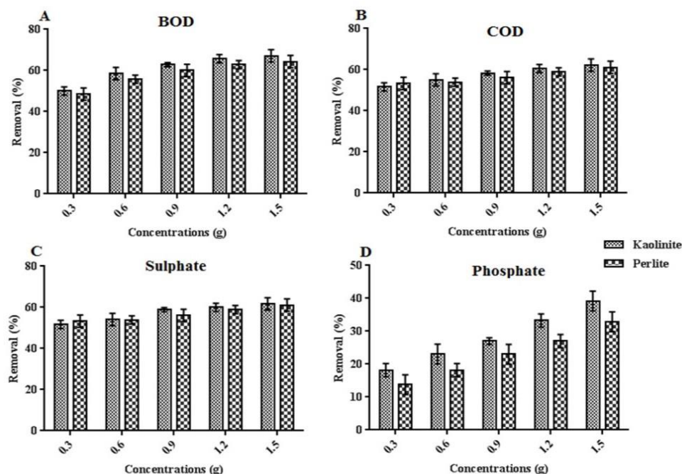
Figure 3. The effects of dosage on the percentage removal of COD, BOD, sulfate, and phosphate using kaolinite and perlite.
